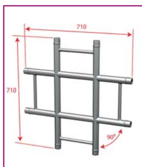
AGDU029-05 Corner joint - 4 directions - 90° - flat
