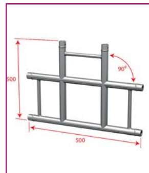
AGDU029-03 Corner joint - 3 directions - 90° - flat
