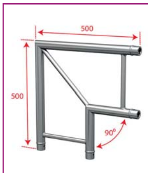
AGDU029-02 Corner joint - 2 directions - 90° - flat
