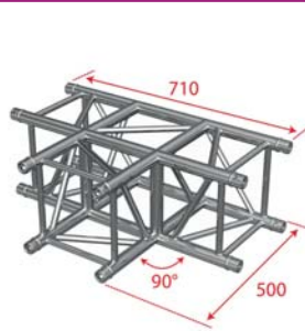
BT-TRUSS QUAT 29 - A017 Quatro angle - 90° - 3 directions
