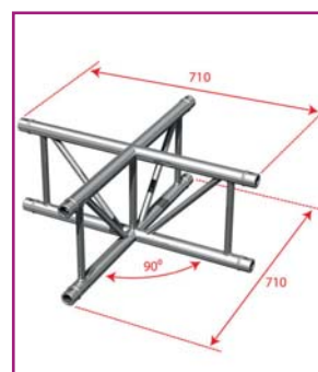
AGDU029-06 Corner joint - 4 directions - 90° - upright
