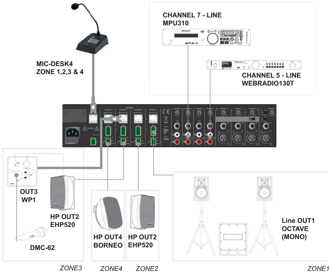
Example of usage of the ZONEAMP4120
